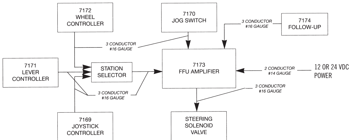
7173 ELECTRONIC FFU SYSTEM DRAWING
