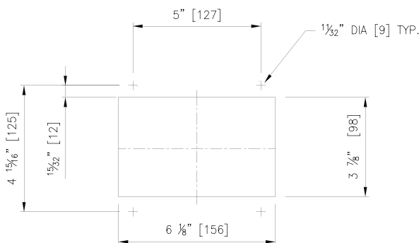
CUT-OUT DIMENSIONS
