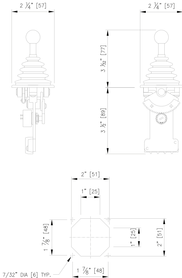
CUT-OUT DIMENSIONS
