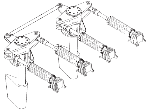
A typical twin rudder steering system with a mechanical tiebar.
