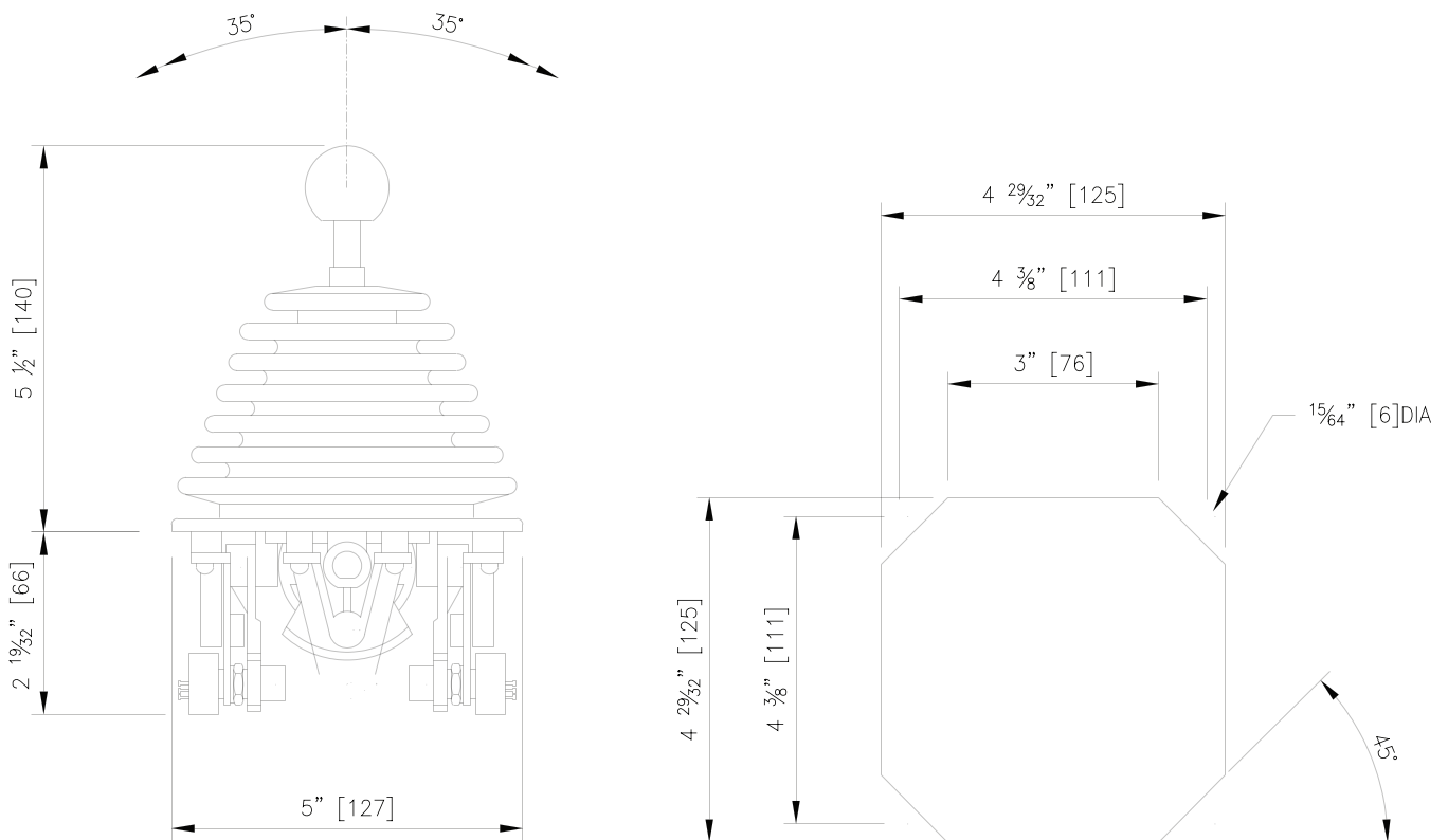
CUT-OUT DIMENSIONS
