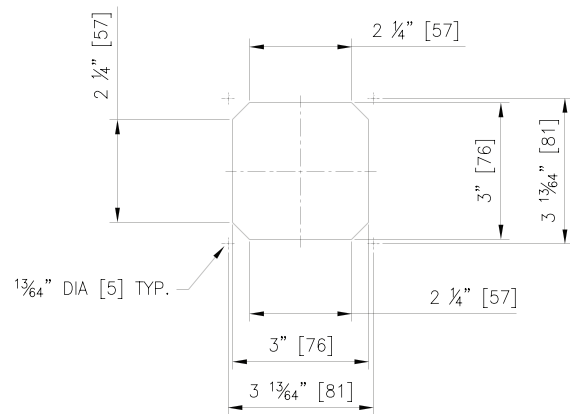
CUT-OUT DIMENSIONS
